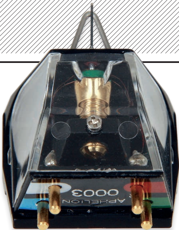
LEFT: Another view of Rega's long boron cantilever and substantial neodymium/iron magnet yoke. The cartridge pins are gold-plated and well spaced to accommodate most tonearm leads/tags
